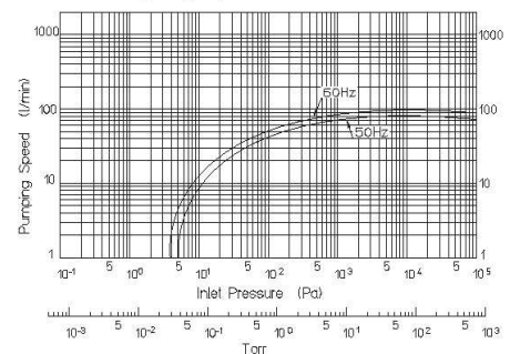
Pumping Speed Curve ISP 90
